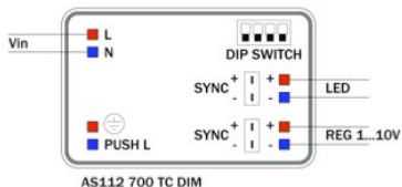
Wiring diagram
