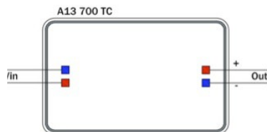
Wiring diagram
